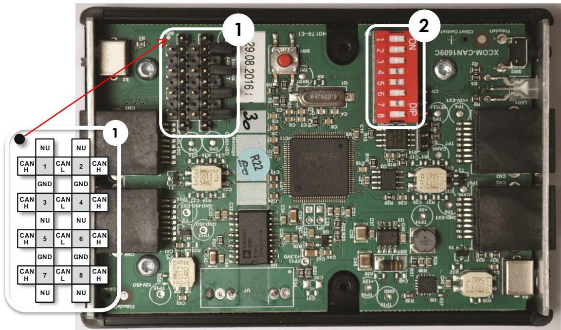
Figure 1: Electronic board inside the Xcom-CAN
