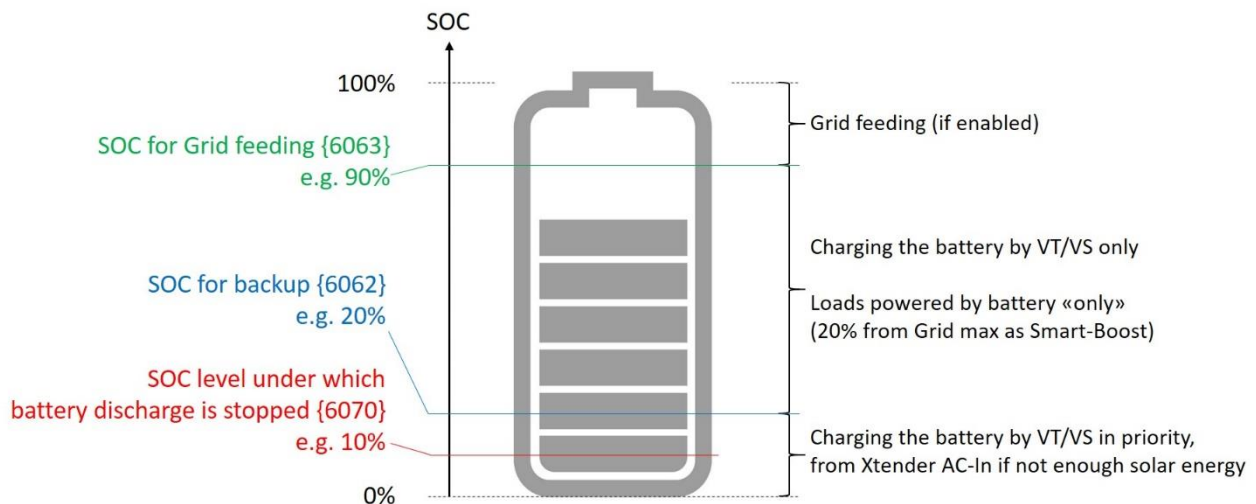
Figure 6: The functioning of a system depending on SOC
