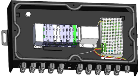
(AC Cable: MAX. 0.75 mm \boxtimes )
