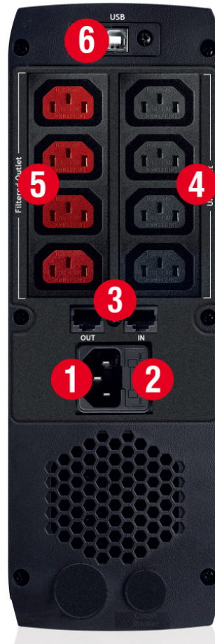
Figure 3 - Rear Side
